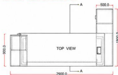
TOP VIEW - 2900 W x 1800 D mm
